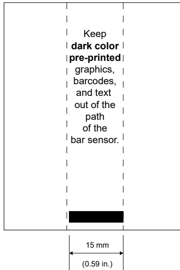
Figure 27 • Label Areas
