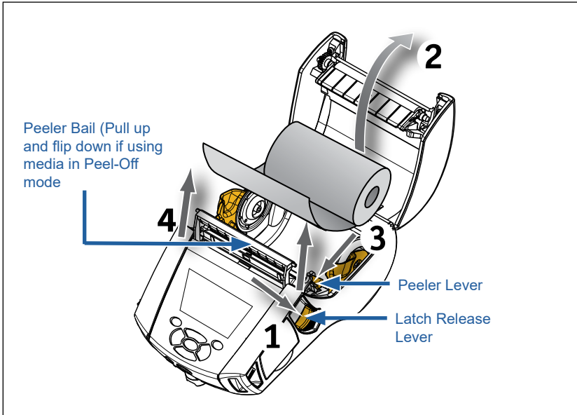
Figure 12 • Activating Peeler Bar (ZQ620 Plus Shown)
