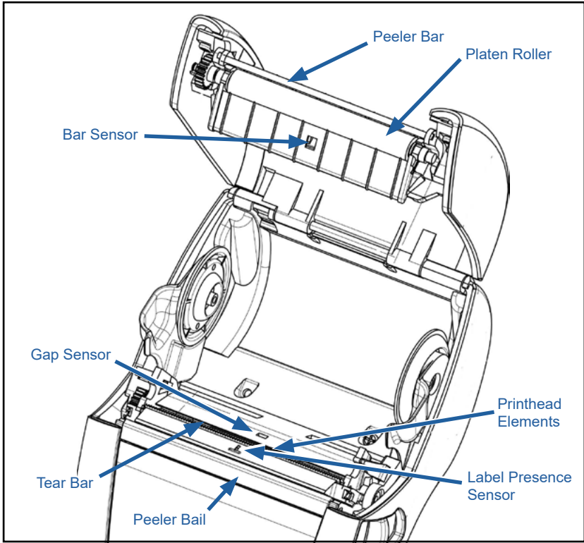
Figure 35 • ZQ6 Plus Cleaning (Linered)
