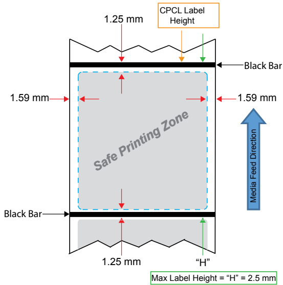
Figure 26 • Black Bar Label Media
