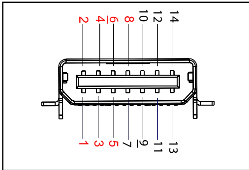
Figure 38 • RS-232C Communication Port
