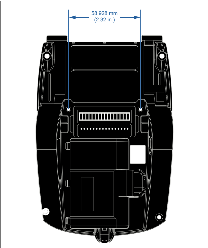
Figure 41 • ZQ620 Plus Mounting Hole Dimensions
