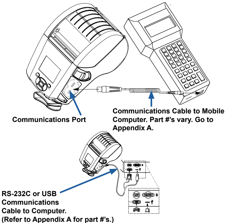
Figure 22 • Communications Options
