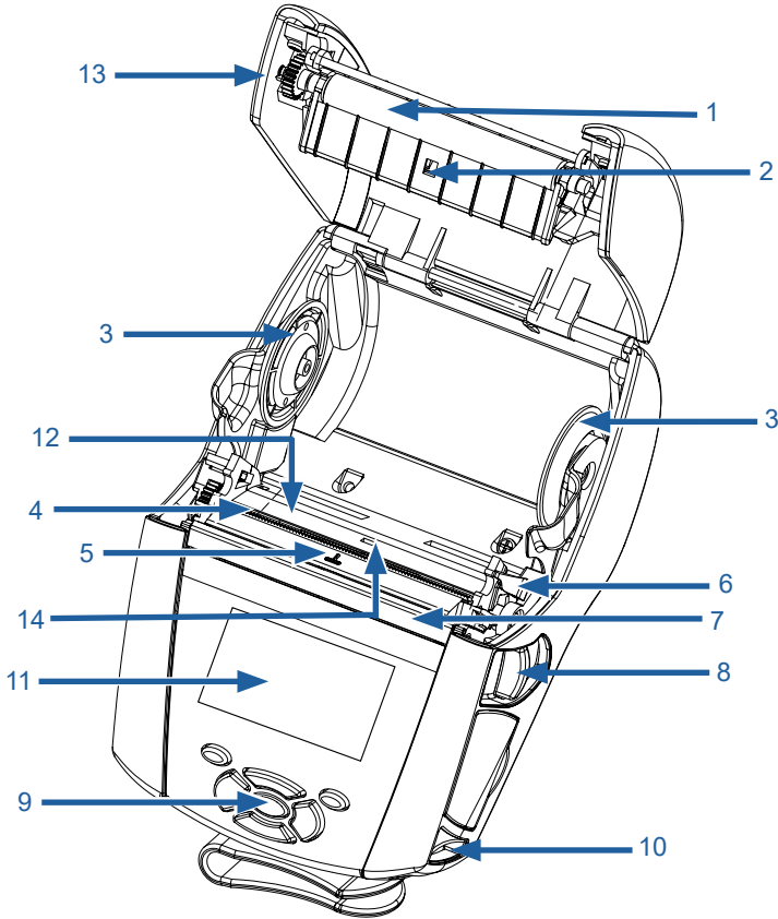
Figure 2 • Overview of Features (ZQ620 Plus Shown).
