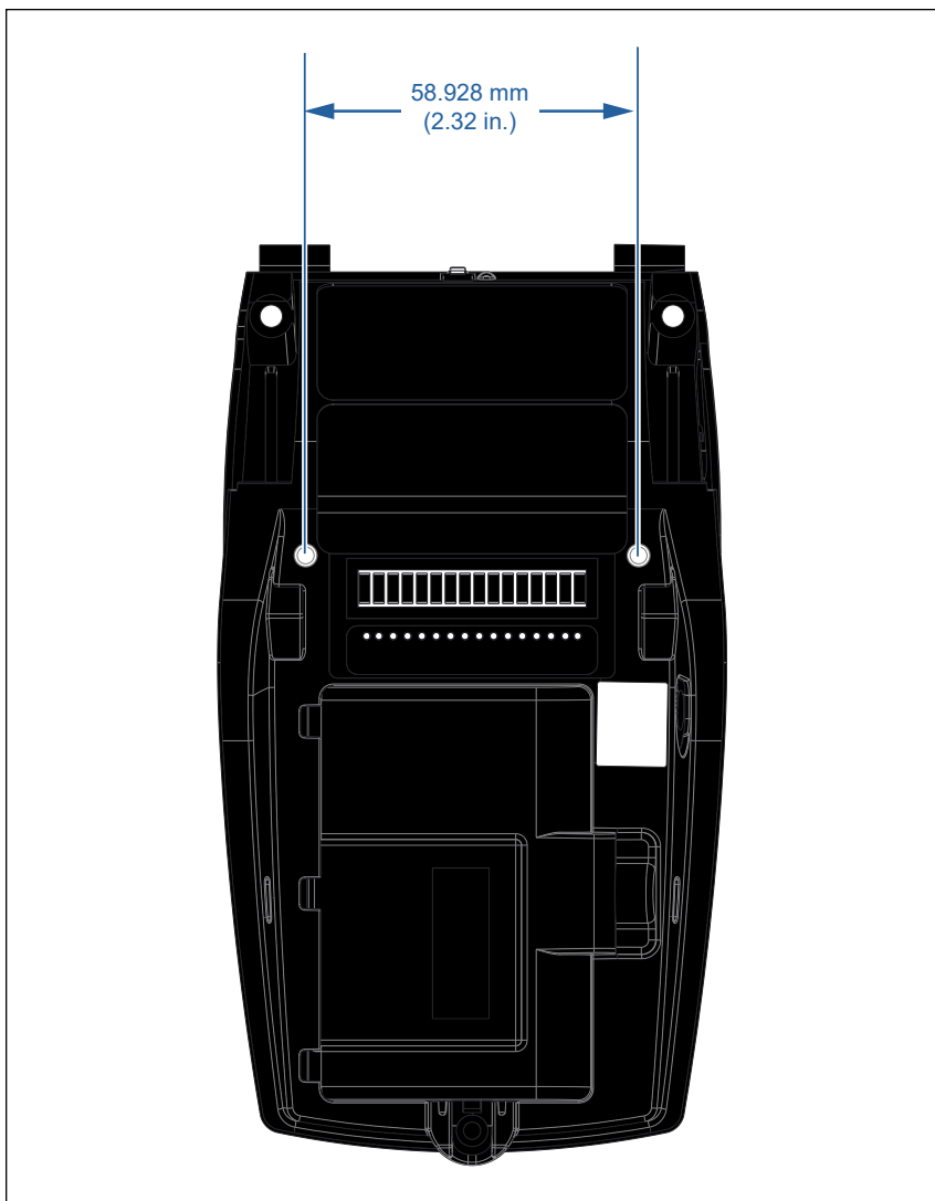
Figure 43 • ZQ610 Plus Mounting Hole Dimensions
