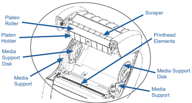
Figure 36 • ZQ6 Plus Cleaning (Linerless)
