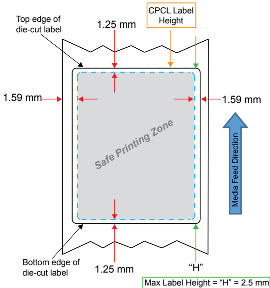
Figure 24 • Gap Media
