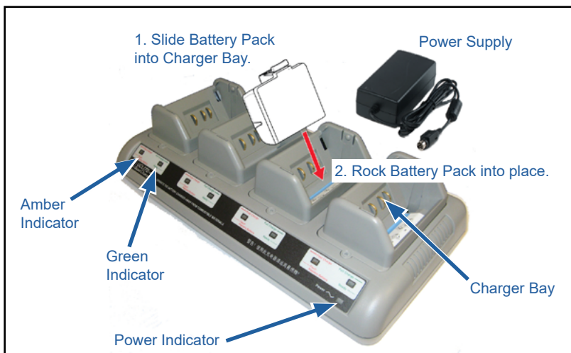
Figure 4 • Quad Charger
