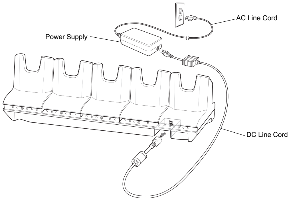
Figure 40 5-Slot Charge Only Cradle Setup
