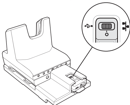
Figure 35 Ethernet Cradle Module Switch
