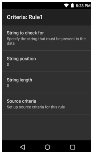
Figure 87 Criteria Screen
