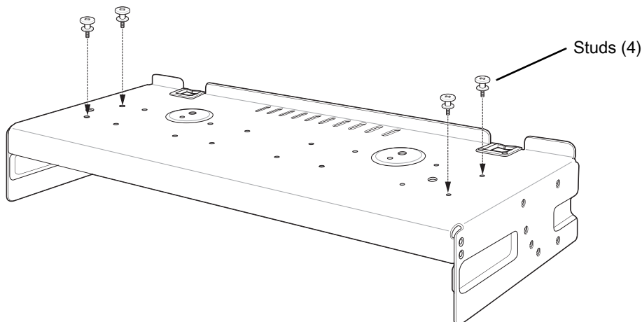
Figure 51 Install Studs
