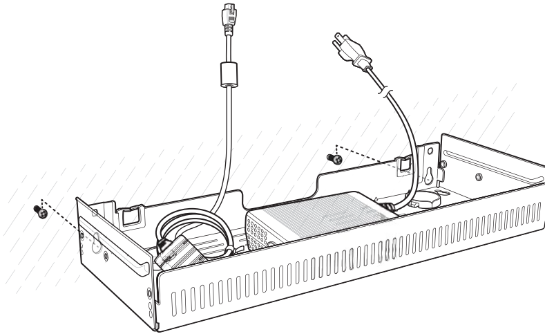
Figure 62 Horizontal Installation
