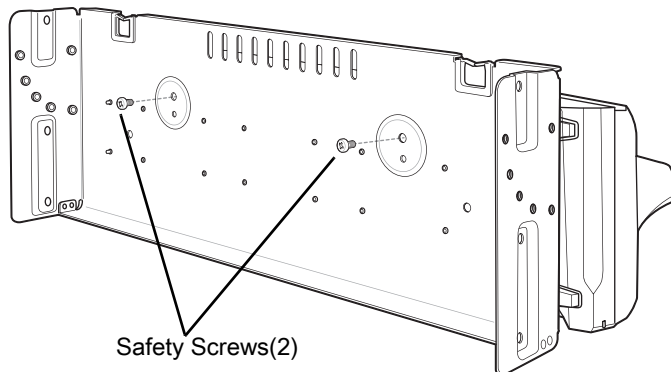
Figure 53 Secure Cradle
