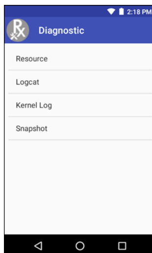
Figure 103 Diagnostic Window
