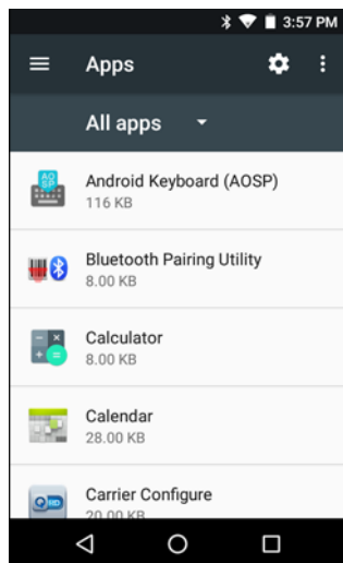
Figure 111 Downloaded Screen
