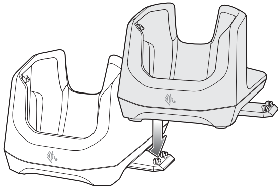
Figure 24 Align Cradles
