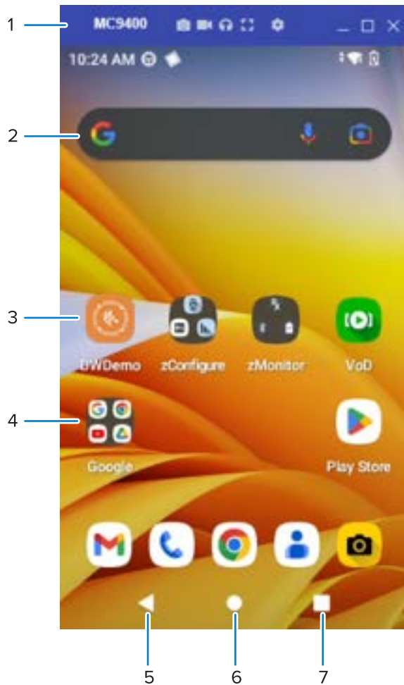
Figure 4 Home Screen
