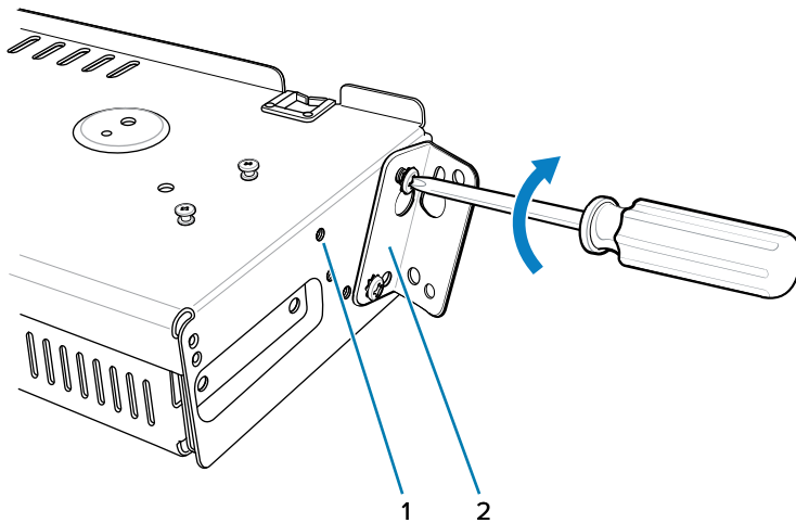
Figure 39 Flange 25° Position (4-Slot Battery Chargers)
