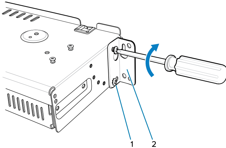
Figure 38 Flange Horizontal Position (5-Slot Cradles)
