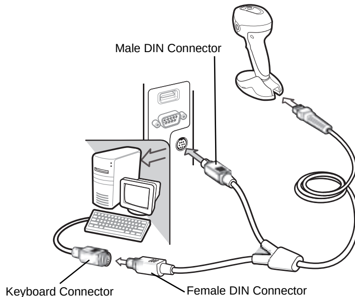
Figure 9-1 Keyboard Wedge Connection with Y-cable
