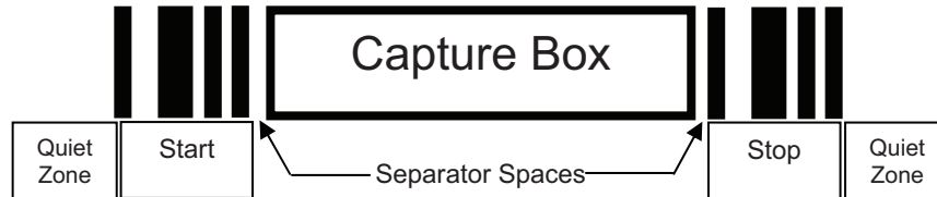
Figure 26 CapCode Structure
