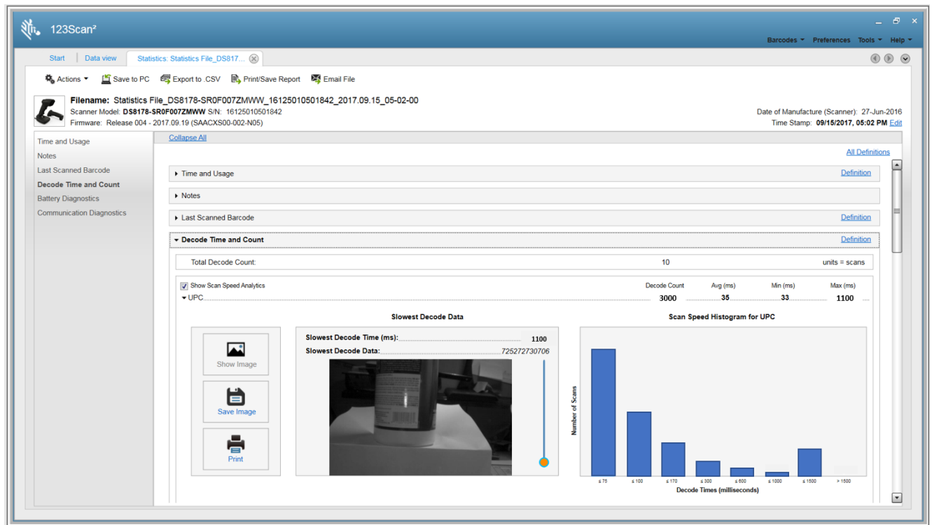
Figure 28 123Scan Statistics Tab - Histogram Data
