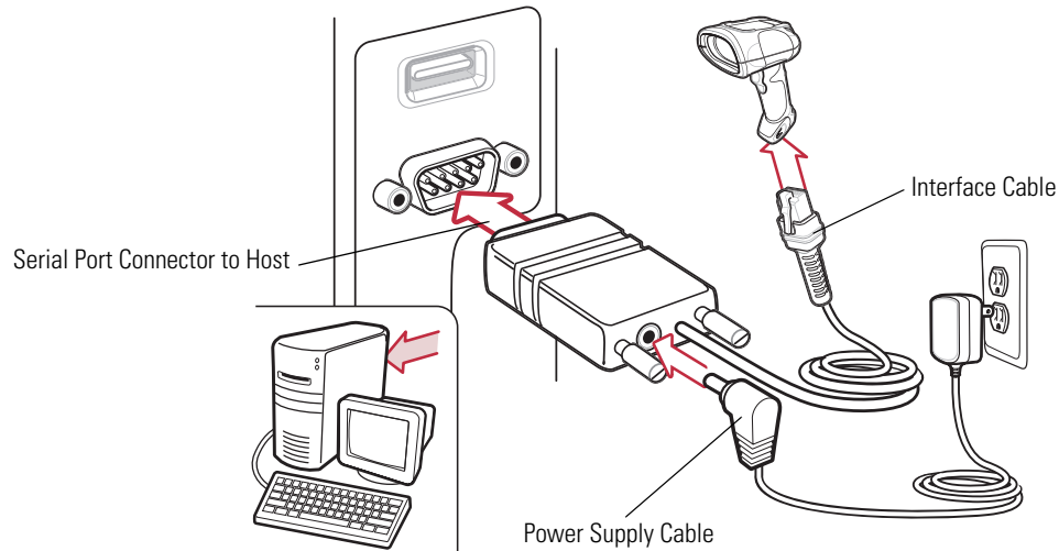
Figure 7-1. RS-232 Direct Connection
