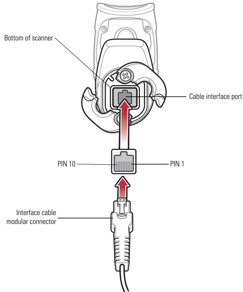
Figure 3-1. Digital Scanner Cable Pinouts
