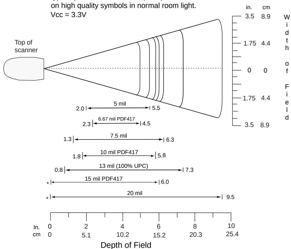
Figure 2-7. DS 3408 Near Focus Decode Zone
