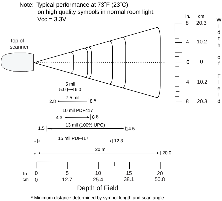
Figure 2-8. DS 3408 Far Focus Decode Zone
