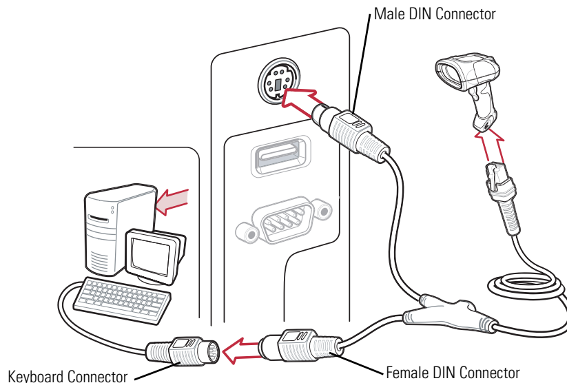
Figure 6-1. Keyboard Wedge Connection with Y-cable
