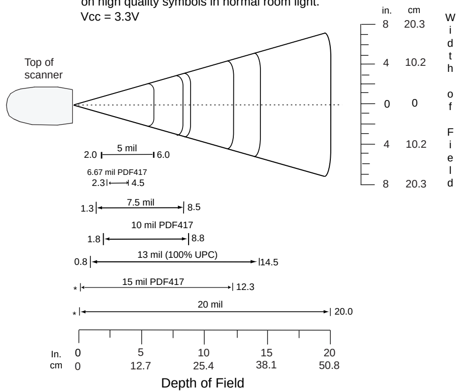
Figure 2-9. DS 3408 Toggle Focus Decode Zone
