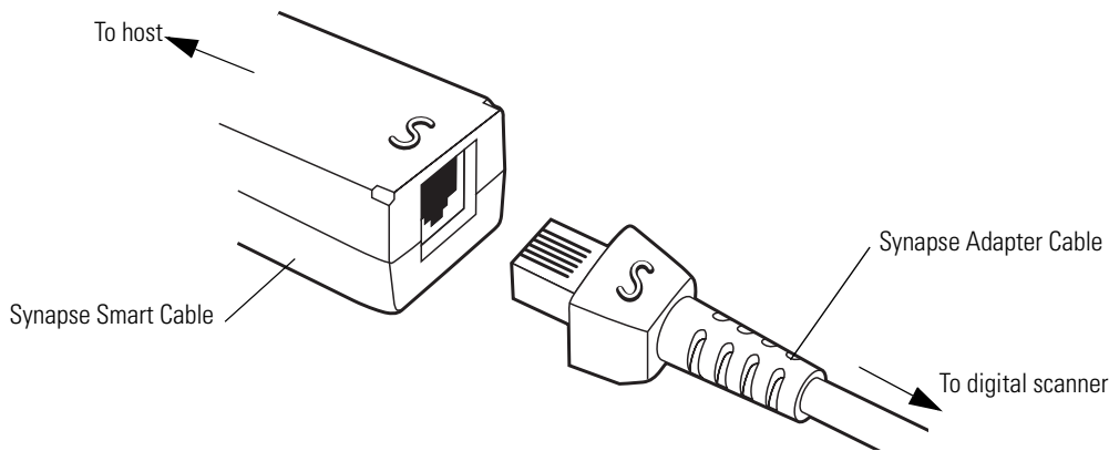
Figure 1-5. Synapse Cable Connection
