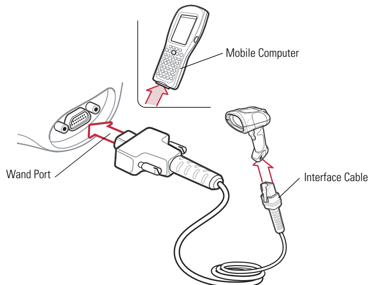
Figure 10-1. Wand Emulation Connection
