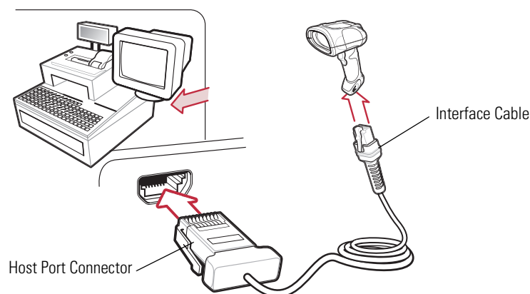
Figure 9-1. IBM Direct Connection
