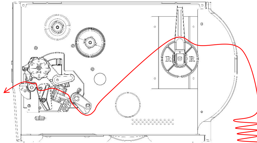
Loading path for fan-fold labels
