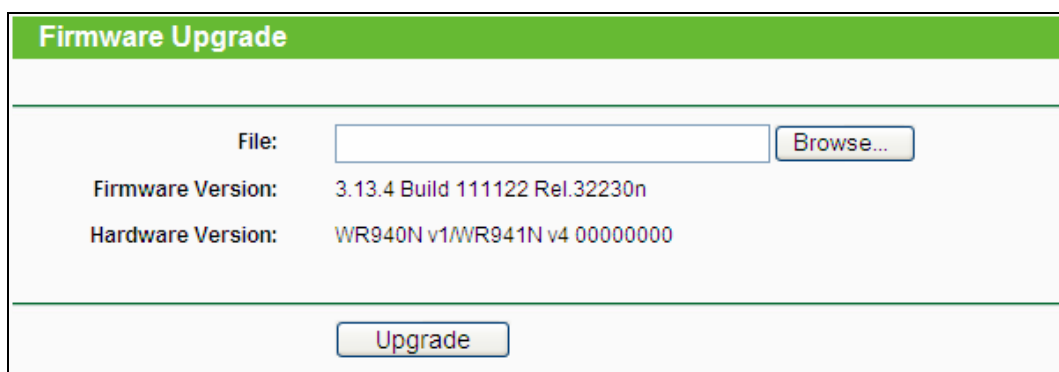
Figure 4-75 Firmware Upgrade
