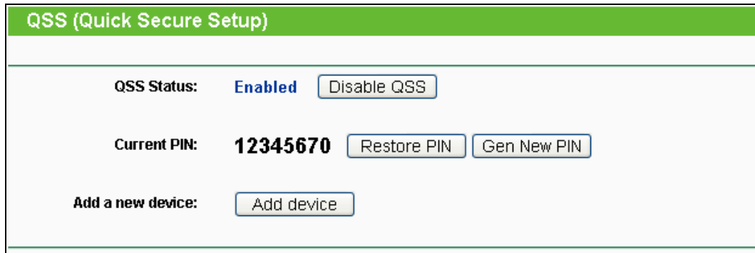
Figure 4-2 QSS
