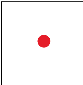
Figure 2-10 Aiming Dot
