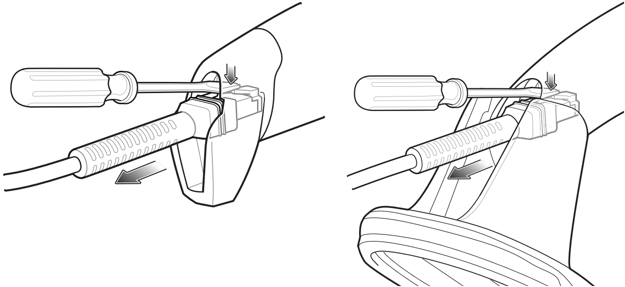
Figure 1-3 Removing the Cable - DS4308 and DS4308P
