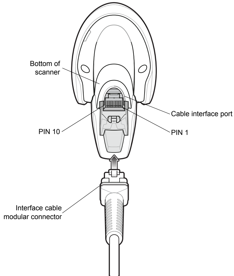
Figure 3-1 Digital Scanner Cable Pinouts
