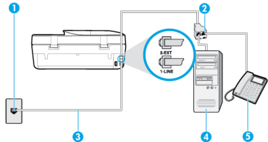
Figure 5-9 Back view of the printer
