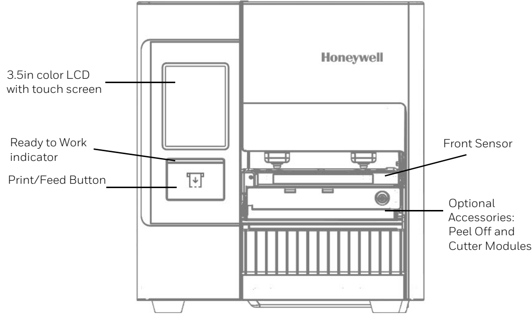
LCD Front View and Features
