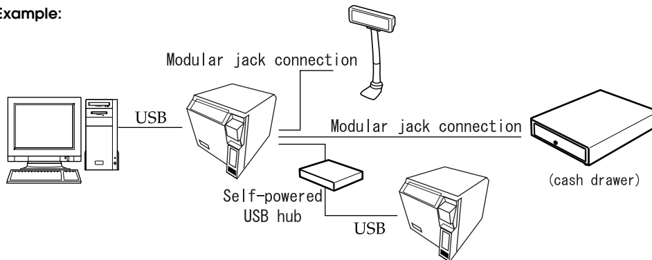
Figure 2-17 USB connection
