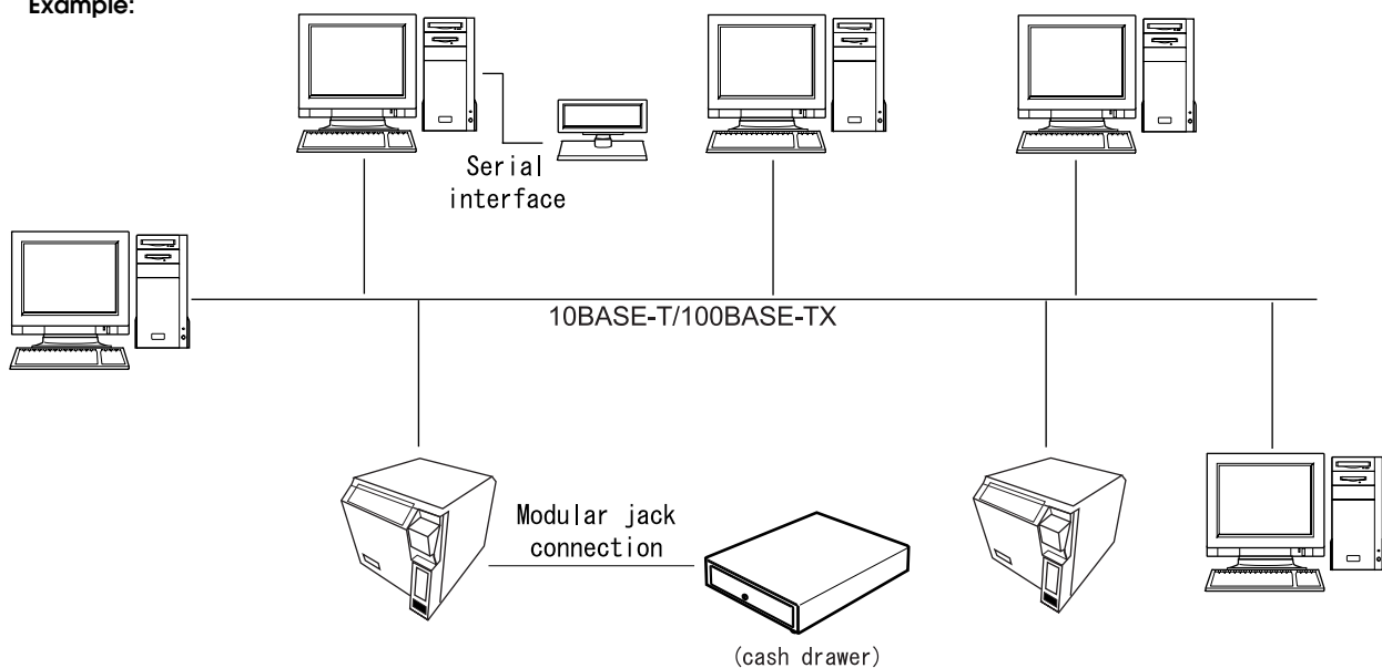
Figure 2-19 Ethernet connection
