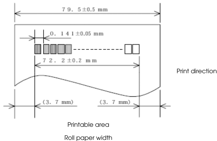
Figure 5-23 Printable area
