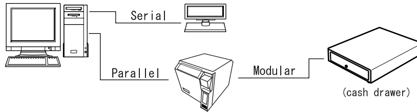
Figure 2-16 Parallel interface connection
