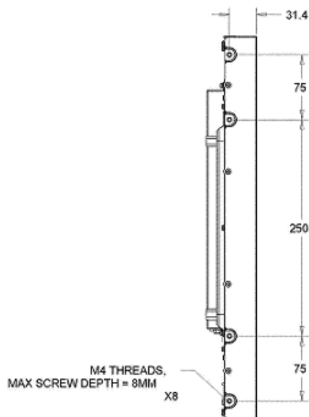
SIDE MOUNT VERTICAL (LEFT/RIGHT)
