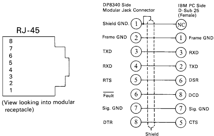
Figure 7-6. Wiring of cable for direct connection between DP8340 and IBM PC serial port
