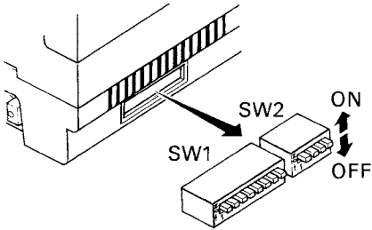
Figure 7-2. Setting of DIP Switch
