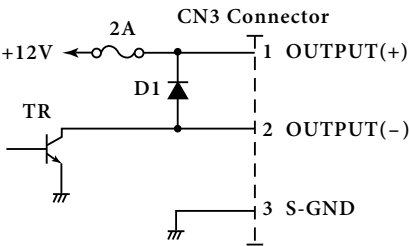
Figure 8-9. Drive Circuit
