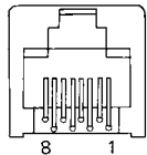
Figure 7-3. Modular Jack Connector
