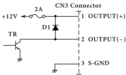
Figure 7-9. Drive Circuit
