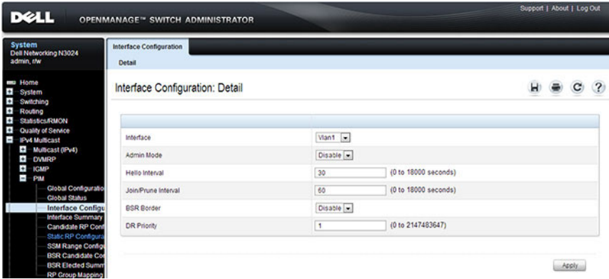
Figure 46-38. PIM Interface Configuration
