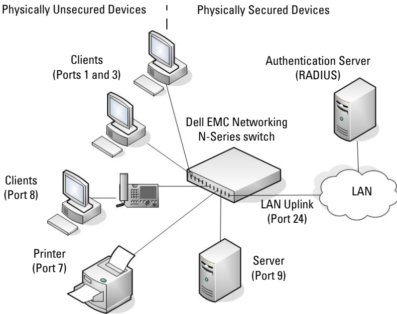
Figure 10-12. 802.1X Example
