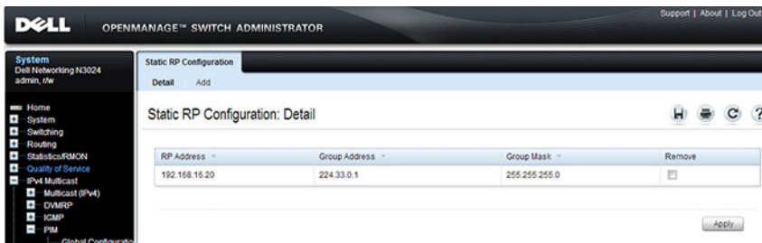
Figure 46-42. Static RP Configuration
