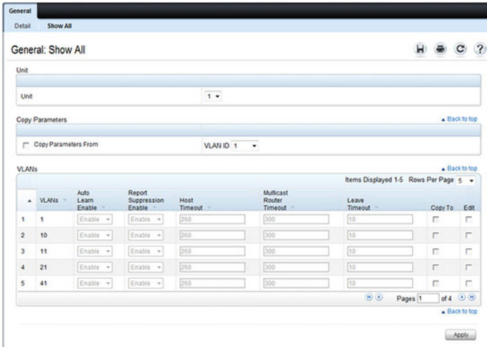
Figure 25-7. Edit IGMP Snooping Settings
