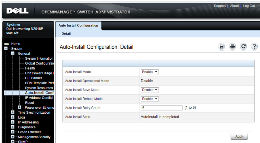
Figure 15-1. Auto-Install Configuration
