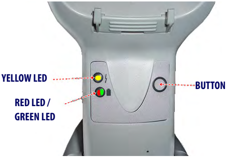
Figure 13. Gryphon Base LEDs
