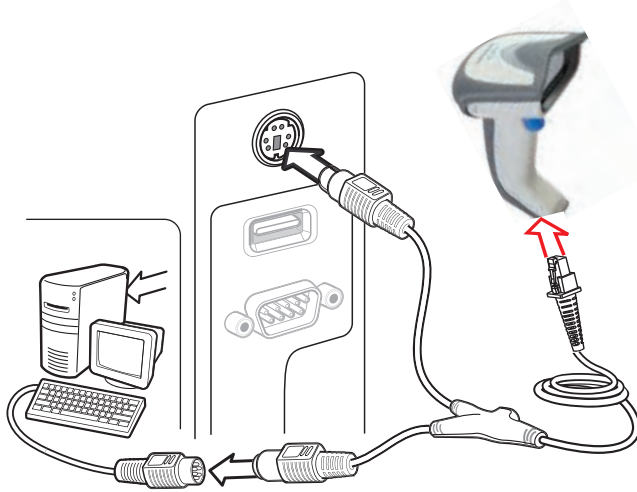
Figure 5. Keyboard Wedge Interface connection
