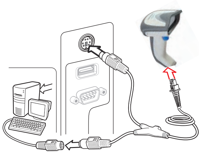
Figure 5. Keyboard Wedge Interface connection
