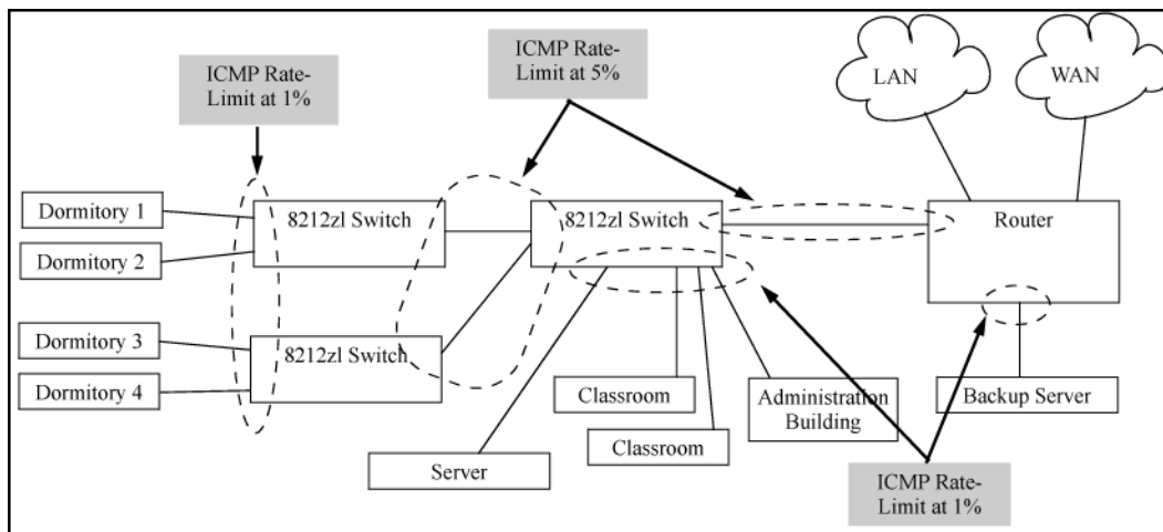
Figure 21: Example: of ICMP rate-limiting
