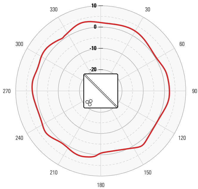
Azimuth - 5 GHz
