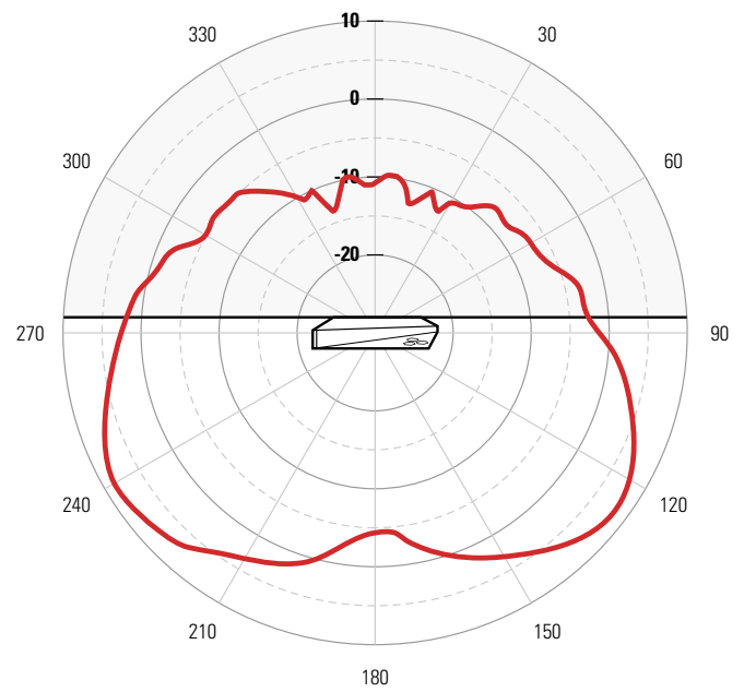
Elevation - 5 GHz
